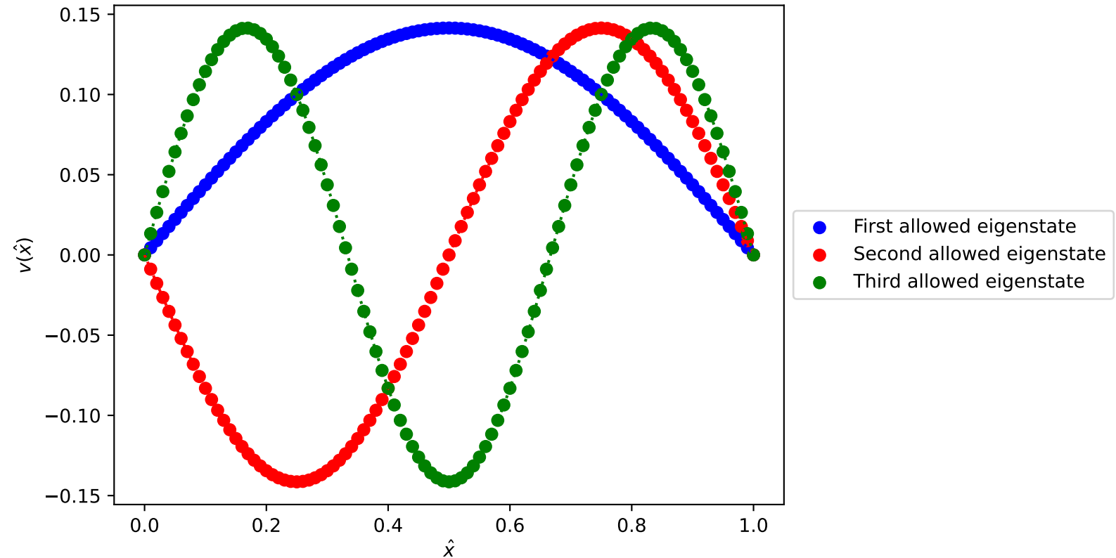
The first three eigenvectors for buckling beam, n=100
